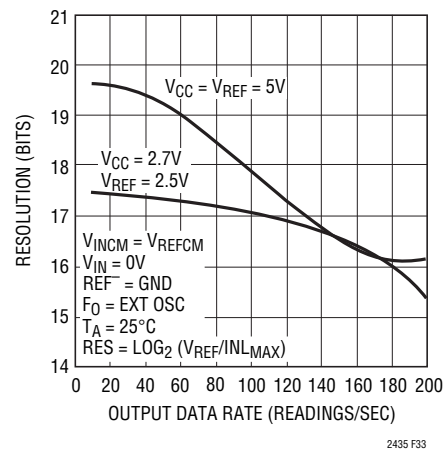
Figure 33. Resolution ( \text{INL}_{MAX} \leq 1\text{LSB} ) vs Output Data Rate and Reference Voltage
