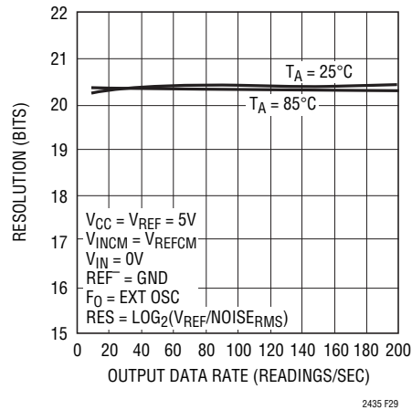
Figure 29. Resolution ( \text{Noise}_{RMS} \leq 1\text{LSB} ) vs Output Data Rate and Temperature
