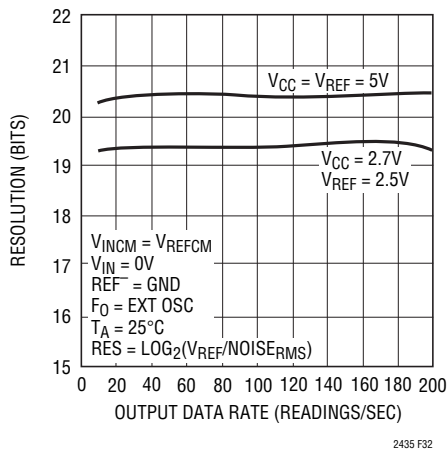
Figure 32. Resolution ( \text{Noise}_{RMS} \leq 1\text{LSB} ) vs Output Data Rate and Reference Voltage
